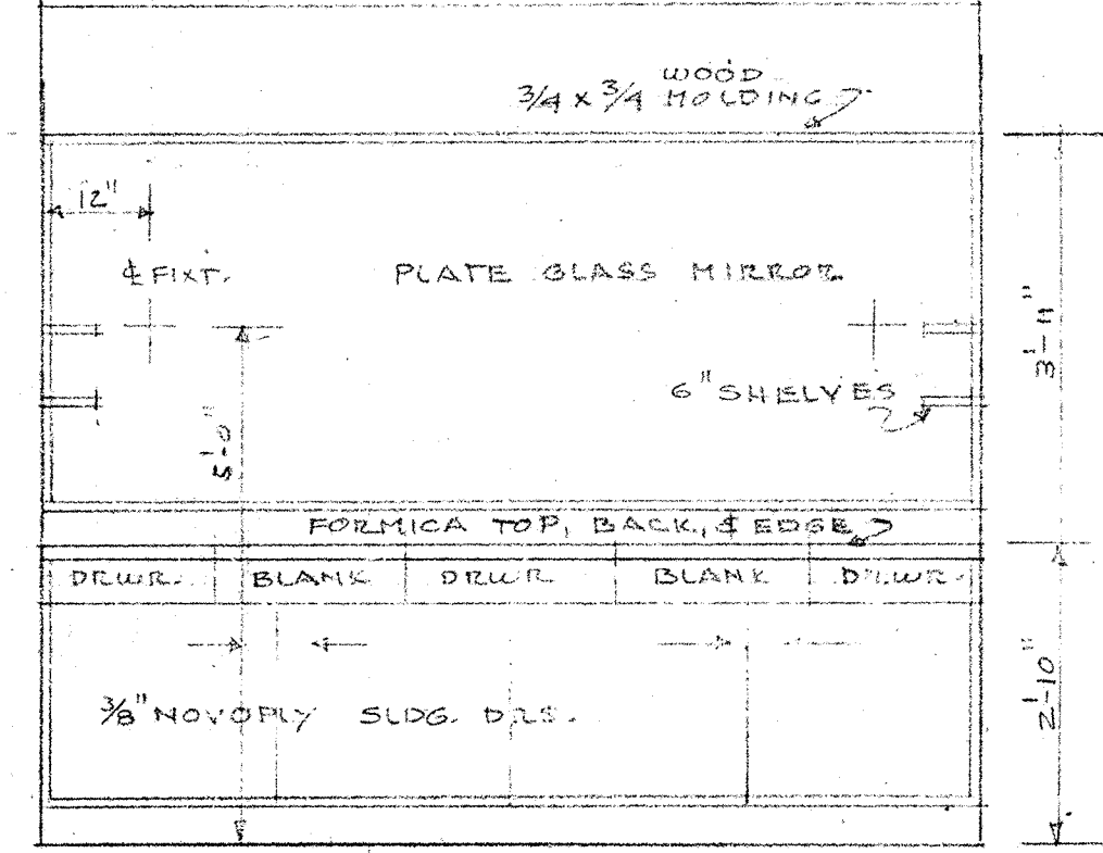
BATH #1 (2 & 3) SIMILAR
